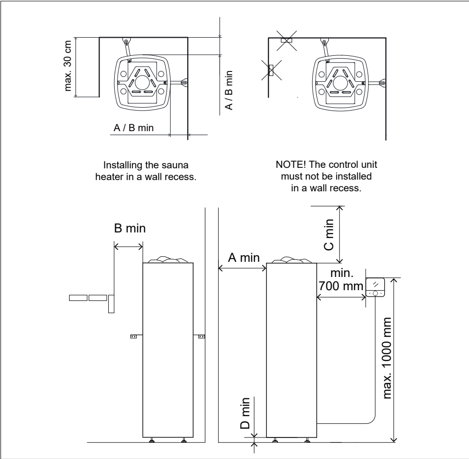
Figure 6.1-1: Minimum safety distances
