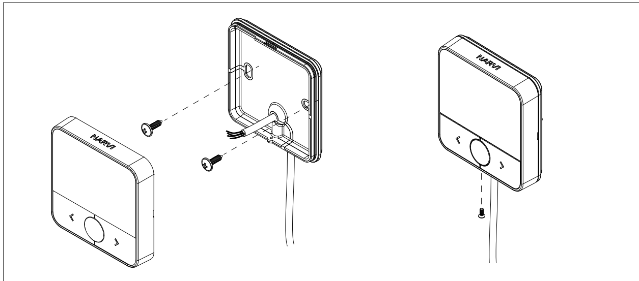
Figure 6.4-1: Installation of the control unit casing
