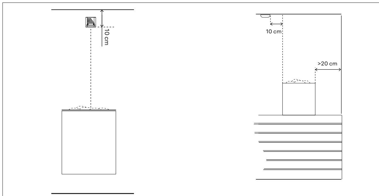
Figure 6.5-1: installation of the temperature sensor
