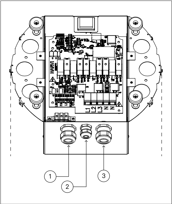
Figure 6.3-1: Cable entries of the connection box
