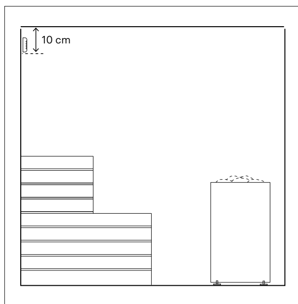
Figure 6.6-1: installation of the humidity sensor
