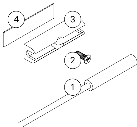
Figure 6.7-1: Door switch set: 1) Door switch with connection cable, 2) Screw 3) Frame switch holder 4) Sticker 5) Magnet 6) Door magnet holder
