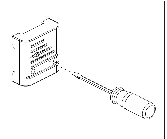
Figure 7.12-1: reactivation of the overheat protector
