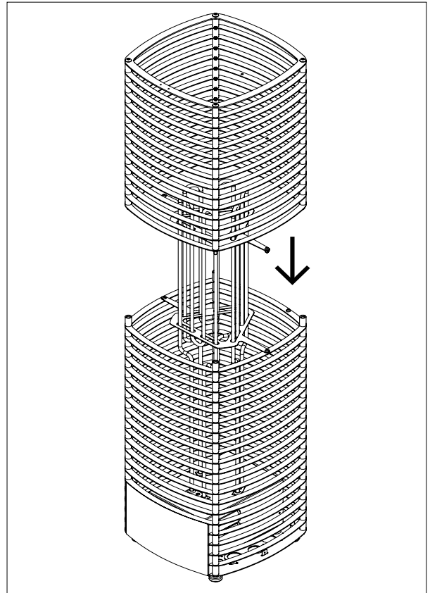
Figure 6.9-3: Installation of the outer casing
