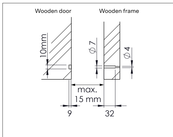
Figure 6.7-3: the embedding of the door switch and the magnet
